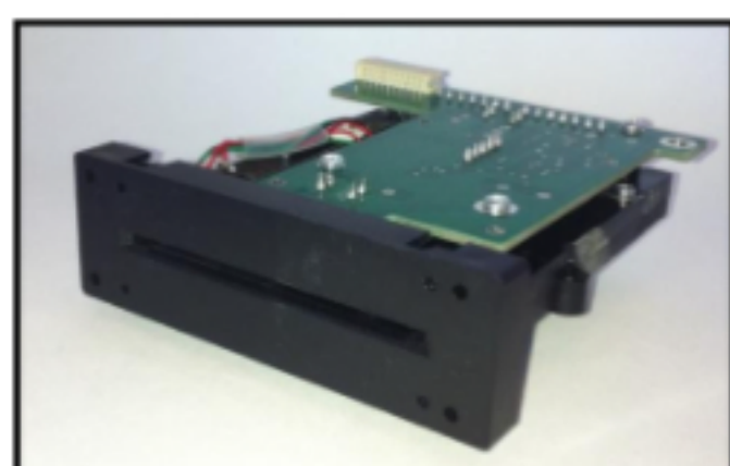
PI60N-120-BST Partial stripe insert card reader Reads 60% of Tracks 1 or 2 or Both Bit/Strobe interface
