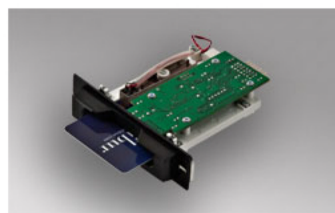
PI65-100/020-BST-MFR Partial stripe insert card reader Reads 65% of track 2 Bit & Strobe interface
