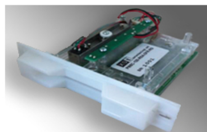
PI65C-120-RSA-DFR-RG Illuminated Red/Green entry slot Reads 65% of tracks 1 & 2 Serial RS-232 interface
